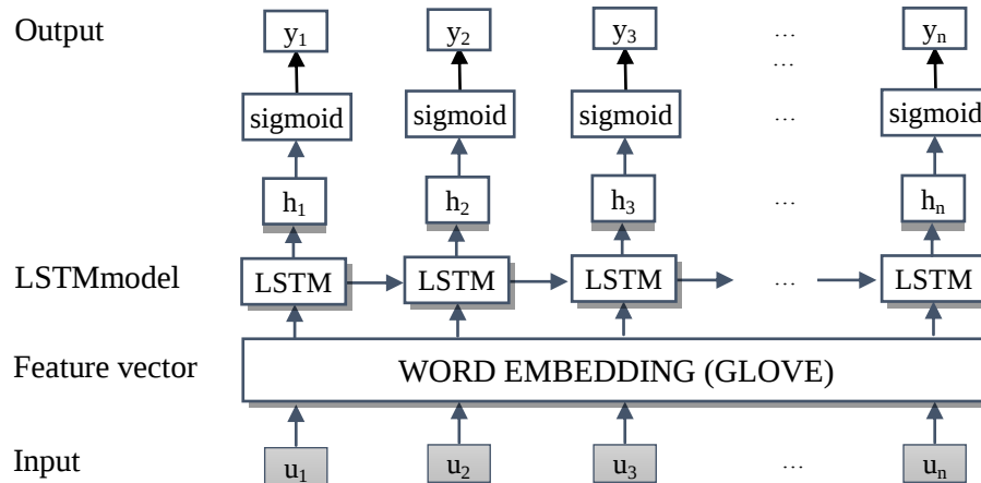
Figure 3. The binary classification model based on LSTM.
