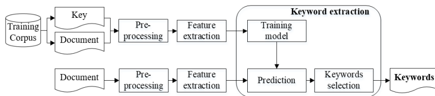
Figure 1. Processing steps for keyword extraction.
