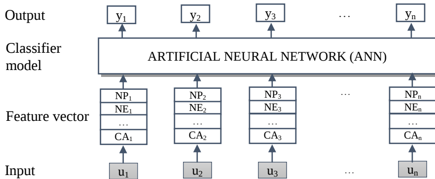
Figure 2. Keyword extraction proposed model.
