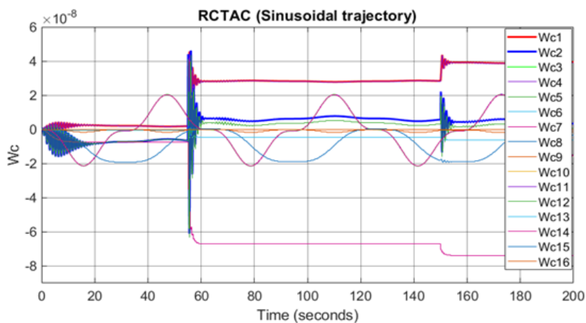
Weighted convergence rate of the Critic network.
