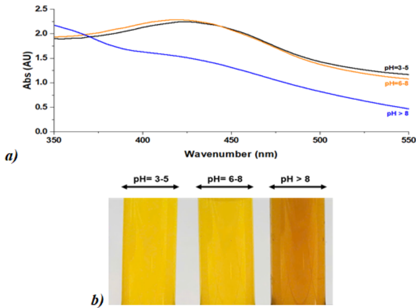
UV-Vis spectra a) and colors b) under different pH conditions of the CMC/NCur films
