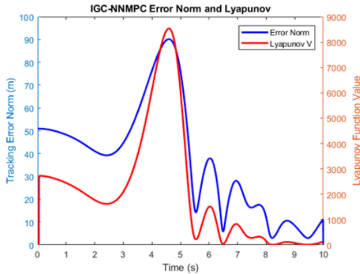
Values of the Lyapunov-Krasovskii function of IGC-NNMPC.
